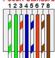
T-568A Standard
