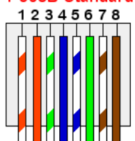
T-568B Standard
