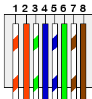
T-568B Standard
