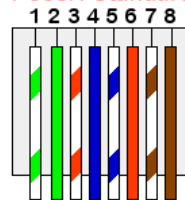
T-568A Standard
